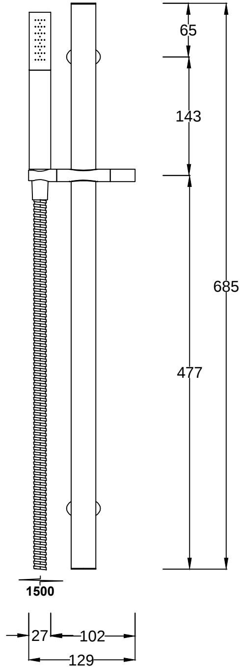
Left View
